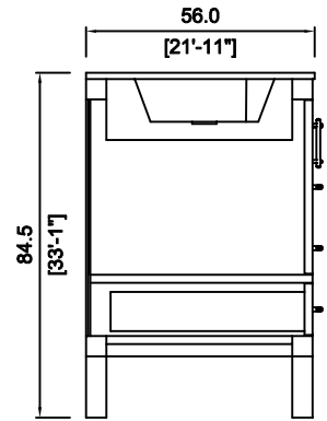
SIDE SECTION
