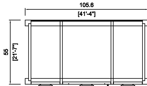
PLAN SECTION
