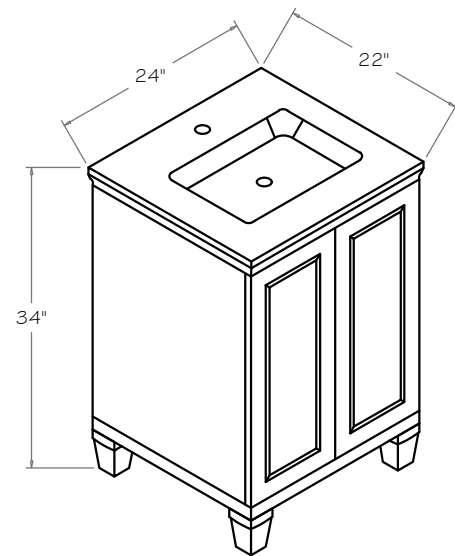
ISOMETRIC VIEW
